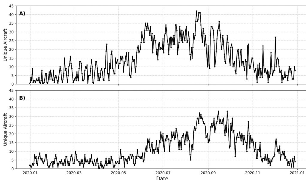
Fig. 2. Line plot illustrating the distribution of unique aircraft activities (CAL FIRE top, USFS bottom) by day for 2020.
