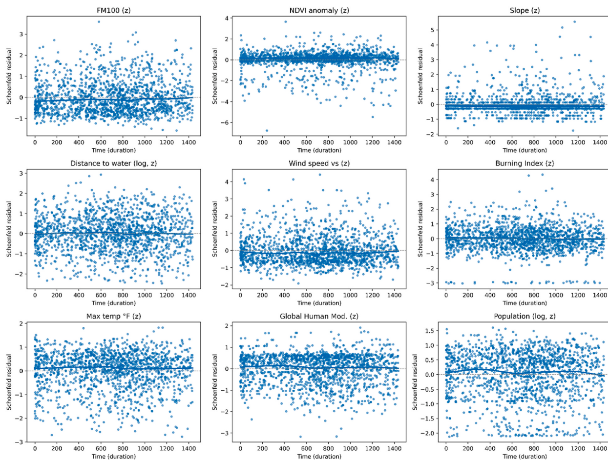
Fig. A5. Schoenfeld residuals for model 1 used to assess the proportional hazards assumption of the dataset.
