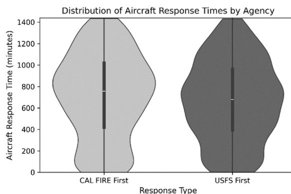
Fig. A8. Violin plots comparing aircraft response times for fires first reached by CAL FIRE versus USFS during the 2020 season.
