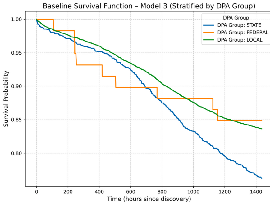
Fig. 5. Baseline survival functions from the DPA-stratified Cox model (Model 3). Curves show the estimated probability that no aircraft has arrived as a function of time since fire discovery for STATE, FEDERAL, and LOCAL Direct Protection Areas.
