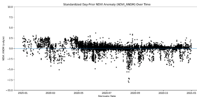
Fig. A3. Standardized day-prior NDVI anomalies for all 2020 fires, showing departures from typical monthly greenness conditions over the fire season.
