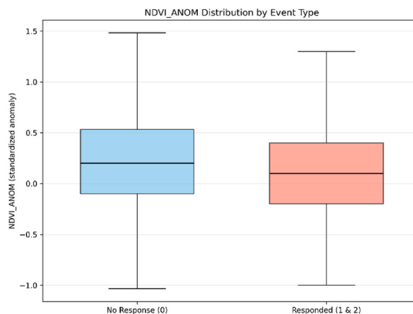
Fig. A4. Boxplots comparing standardized NDVI anomalies for fires with no aerial response versus those that received an initial aircraft response.
