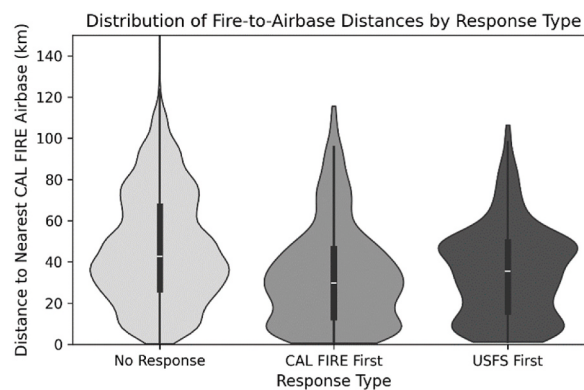
Fig. A2. Violin plots showing distances from fires to the nearest CAL FIRE airbase, grouped by response type (No Response, CAL FIRE first, USFS first).
