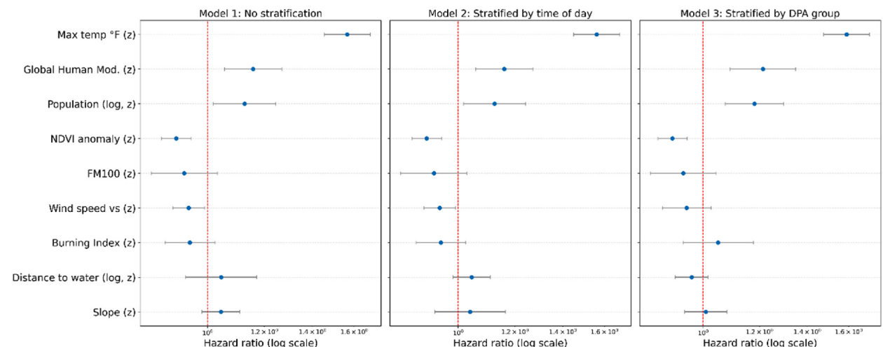
Fig. A7. Hazard ratios and 95% confidence intervals from three Cox proportional hazards models evaluating factors influencing the timing of initial aircraft dispatch. Each panel corresponds to a different model specification: (left) Model 1 with no stratification, (center) Model 2 stratified by time of day (morning, afternoon, night), and (right) Model 3 stratified by DPA. The red dashed vertical line at HR = 1 denotes the null effect.
