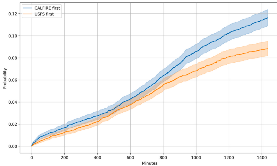
Fig. 4. CIFs estimated using the Aalen–Johansen method for initial aircraft response to wildfires in California during 2020. The blue line represents the probability over time that CAL FIRE is the first to respond; the orange line represents USFS. Shaded areas indicate 95% confidence intervals. Time is measured in minutes from fire discovery.
